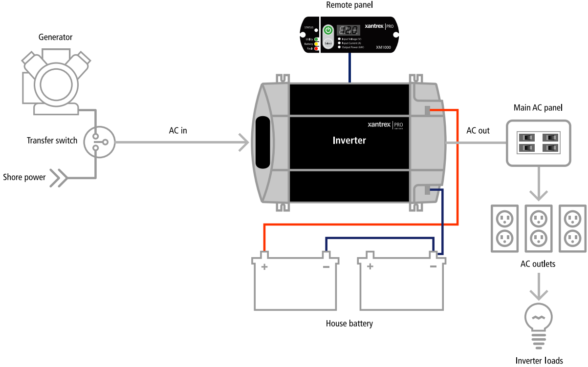
Figure 2: Sample electrical system without an inverter sub-panel
