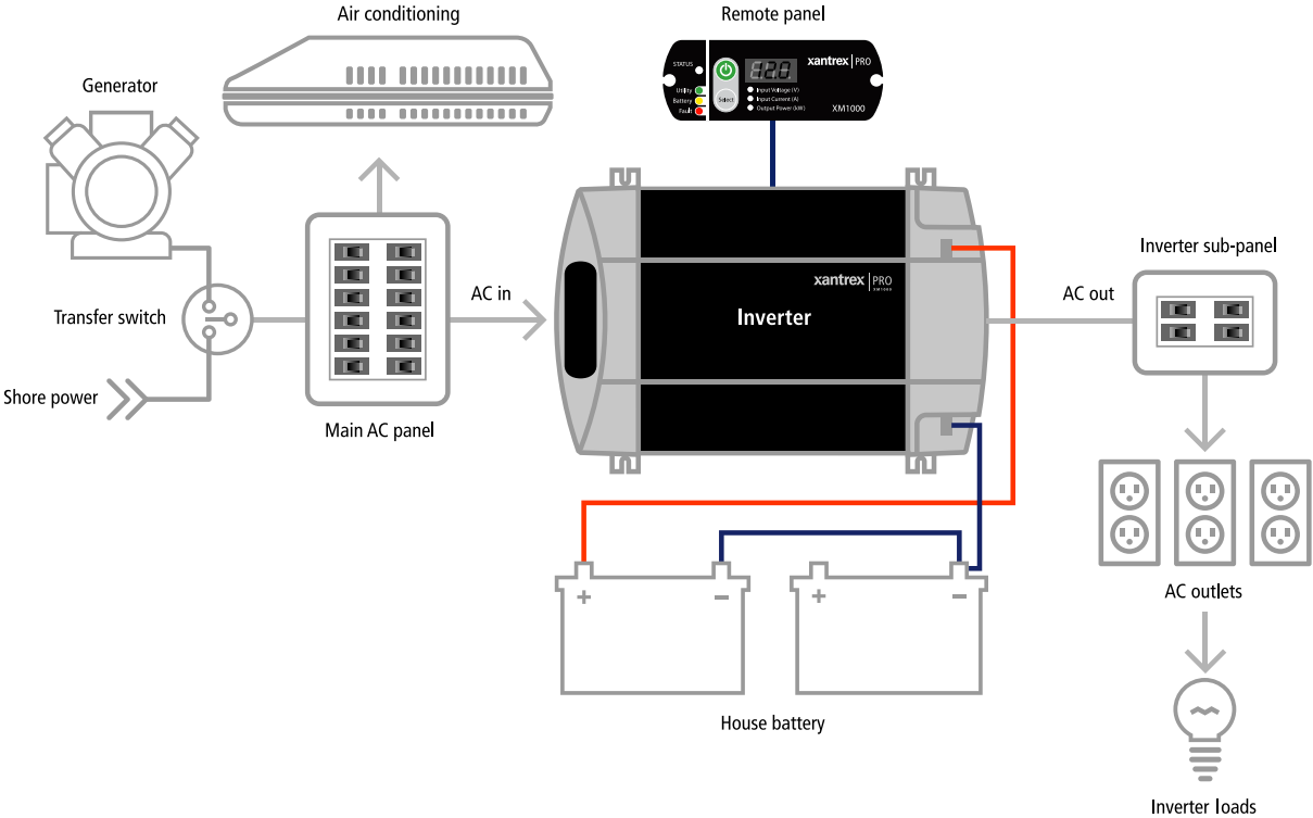
Figure 1: Sample electrical system with an inverter sub-panel
